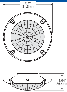
FSP-L7 dimensions
