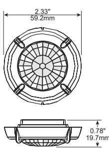
FSP-L3 dimensions
