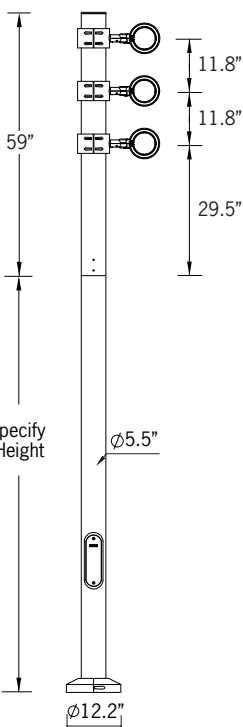
Mounting Detail
