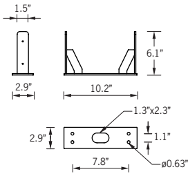
Mounting Detail
