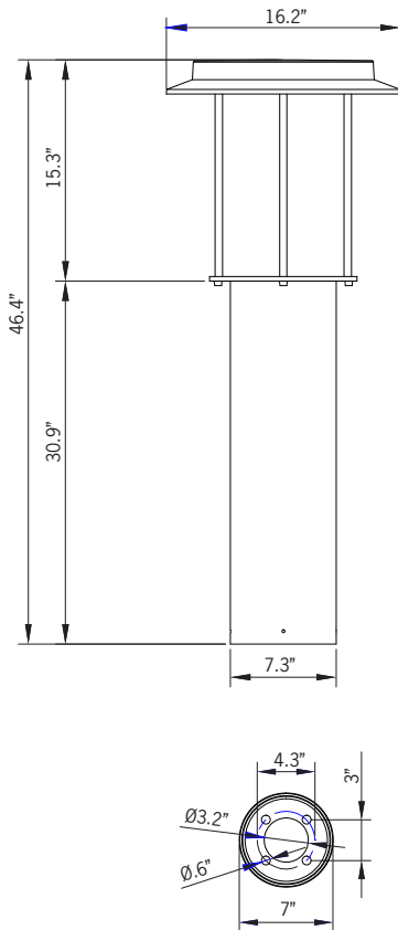
Mounting Detail
