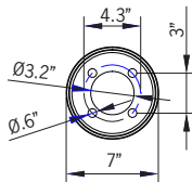
Mounting Detail
