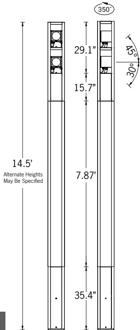
Mounting Detail
