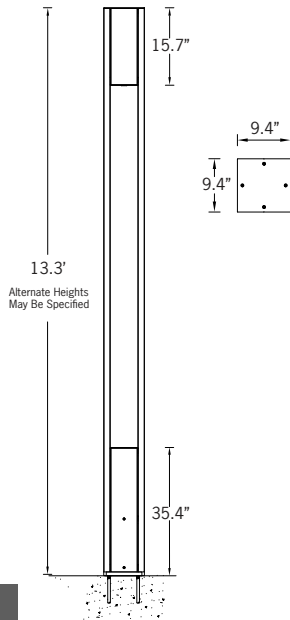
Mounting Detail
