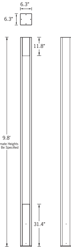
Mounting Detail
