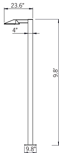
Mounting Detail
