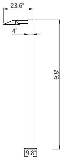
Mounting Detail
