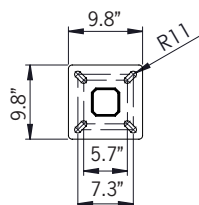
Mounting Detail
