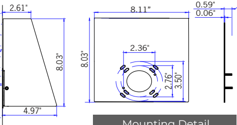
Mounting Detail
