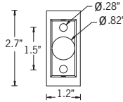
Mounting Detail
