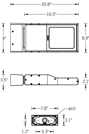
Mounting Detail
