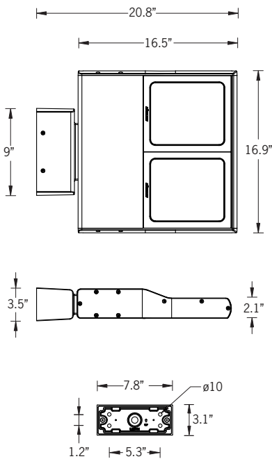
Mounting Detail
