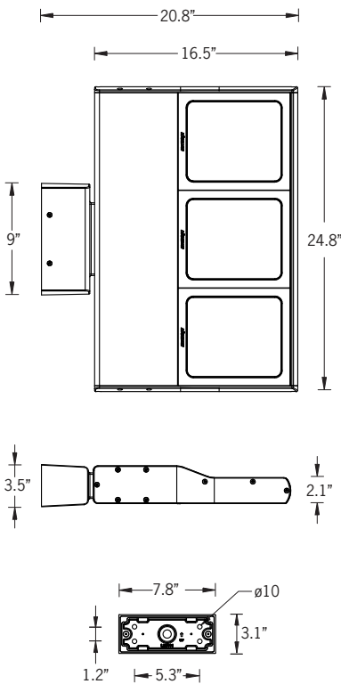
Mounting Detail
