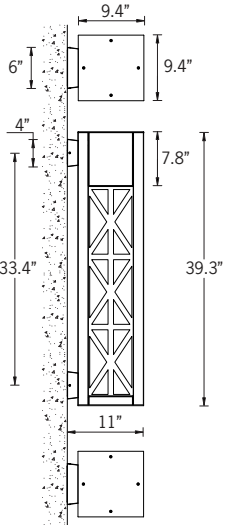
Mounting Detail
