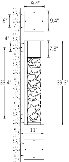
Mounting Detail
