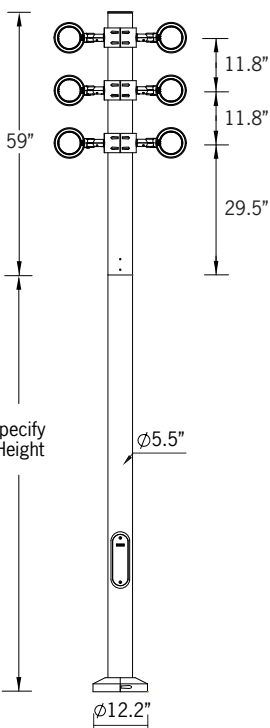
Mounting Detail
