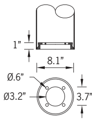
Mounting Detail
