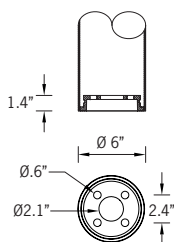
Mounting Detail
