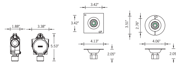
A90521 Catenary Suspension
